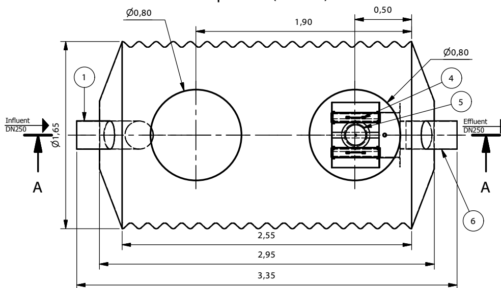
Top View ( 1 : 30 )
