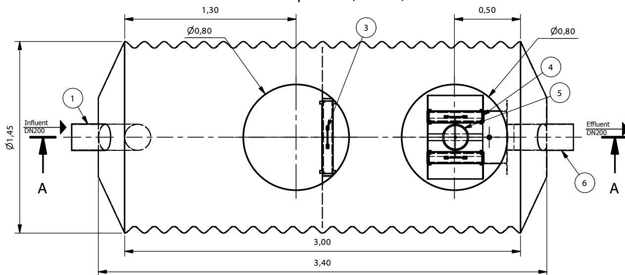
Top View ( 1 : 25 )
