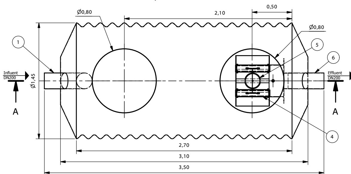
Top View ( 1 : 25 )
