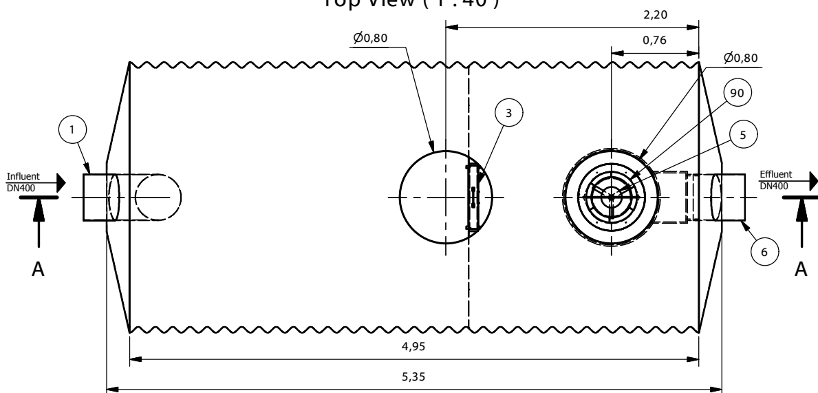
Top View ( 1 : 40 )
